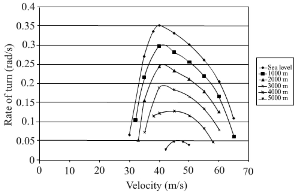
Fig.9.6a Turning performance of a piston engine airplane - variation of rate of turn ( \dot{\psi} )
