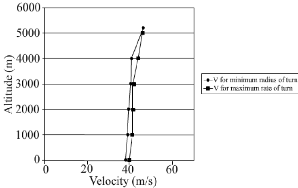
Fig.9.6e Turning performance of piston engine airplane – variations of V_{rmin} and V_{\psi max} with altitude
